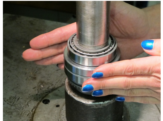
5. Press down the small tapered roller bearing in small steps until correct preload is achieved. Not too tight and no backlash.
