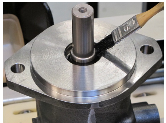
18. Lubricate the sealing surface on the shaft before assembling the shaft seal.
