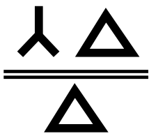
12 Pulse Transformer Configuration
