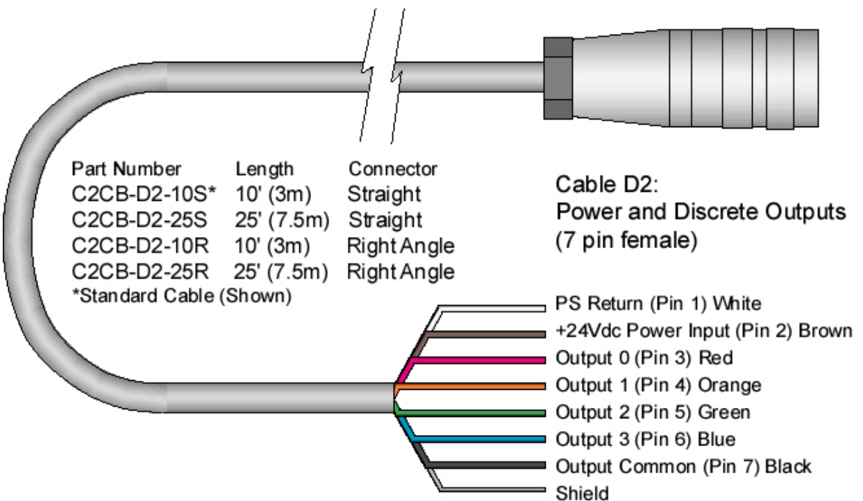
Figure 7: CS24D standard cables. (Order CS24D-xx Kit to include with sensor).
