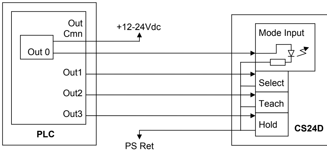
Figure 5: Example Interface: PLC sourcing-type outputs to CS24D inputs
