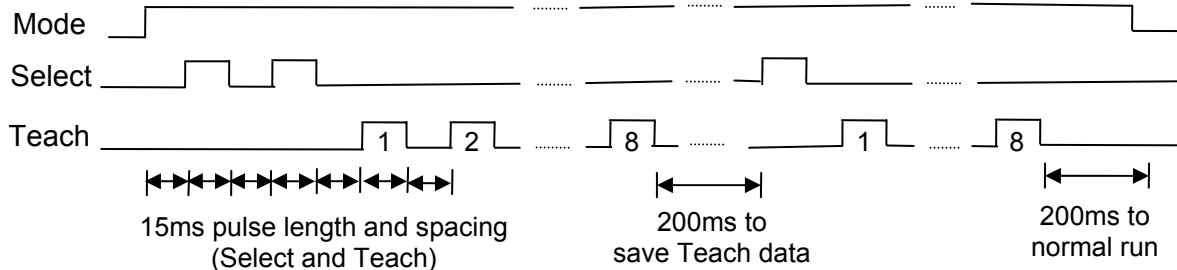
Figure 8: Teach Mode Timing
