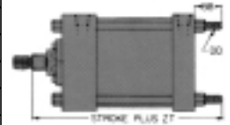
Tie Rods extended cap end Model 52-B (NFPA MX2)
