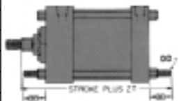
Tie Rods extended both ends Model 54-B (NFPA MX4)
