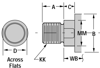
Style No. 2-Standard Threaded on Turndown Section
