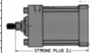
Square Cap Model 64-B (NFPA ME4)
