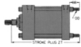
Tie Rods extended cap end Model 52-B (NFPA MX2)
