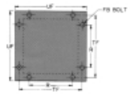
Square Flange/Cap End Model 66-B (NFPA MF6)
