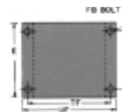
Rectangular Flange/Cap End Model 62-B (NFPA MF2)
