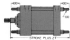
Tie Rods extended both ends Model 51-B (NFPA MX1)
