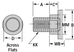
Style No. 6 Studded Rod End
