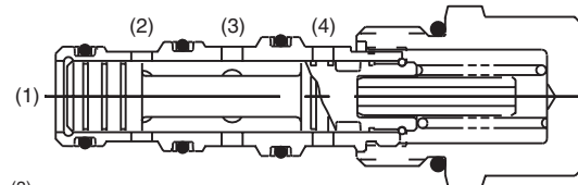
"C" SPOOL - DH103C
