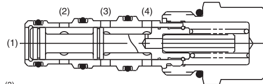
"B" SPOOL - DH103B
