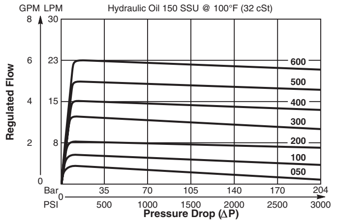
Regulated Flow vs. Pressure Drop (Through cartridge only)
