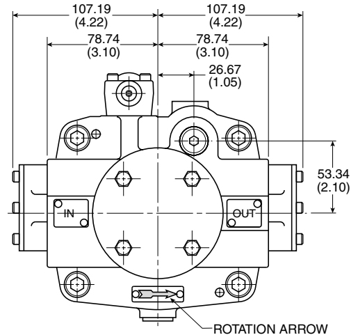
Rear View
