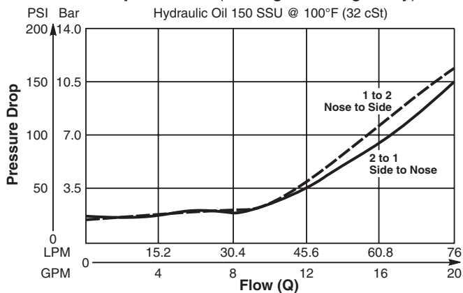
Pressure Drop vs. Flow (Through cartridge only)
