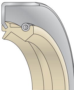
Parker Oil Seal
