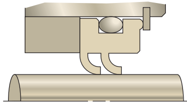
Formed Lip
