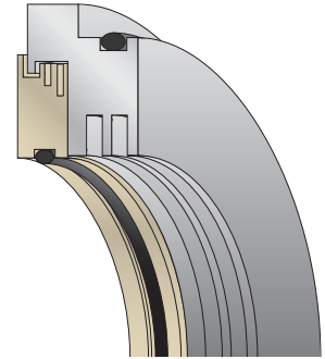
ProTech Bearing Isolator
