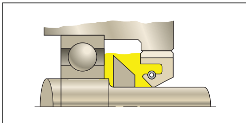
Figure 12-2. Standard lip seal with internal DS sling to protect lip from lubricant surge.
