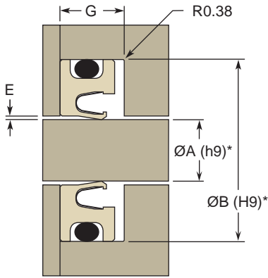
Rotary Seal
