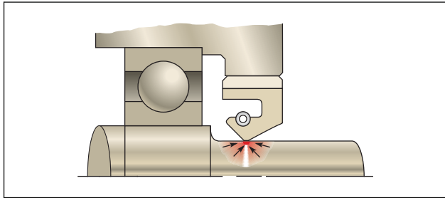
Figure 2-9. Internal Pressure
