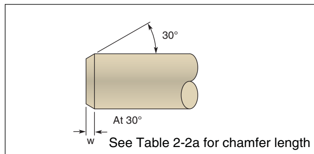
Figure 2-7. Shaft Profile
