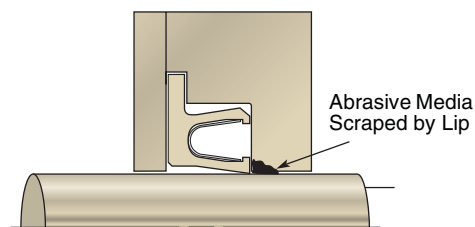
Flanged Scraper Lip at ID
