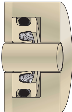
Rotary Housing
