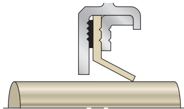
Machined Lip
