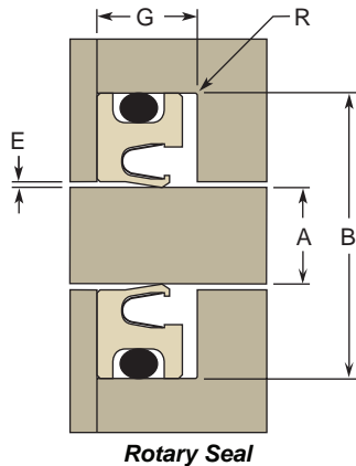
Rotary Seal
