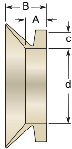
Profile Dimensions
