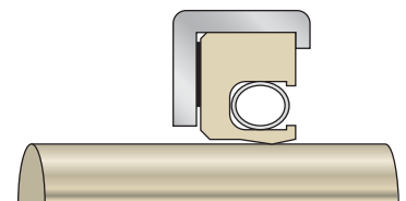
Chamfered Lip
