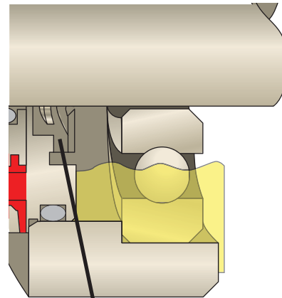
Severe Splash Groove
