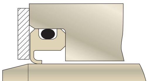
FlexiLip Application
