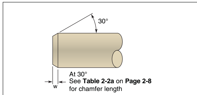
Figure 2-18. Shaft Profile
